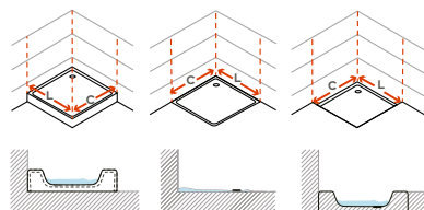
base shower tray
